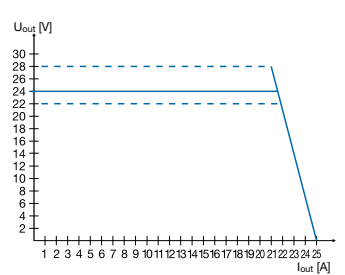
CP-C 24/20.0
