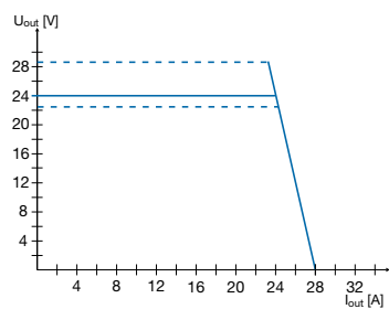
CP-E 24/20.0
