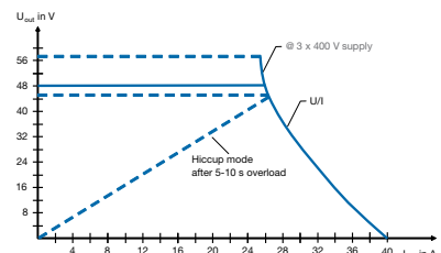
CP-T 48/20.0
