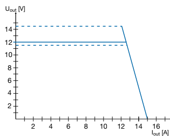
CP-E 12/10.0
