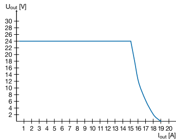
CP-S 24/10.0
