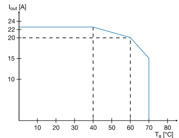
CP-S 24/20.0, CP-C 24/20.0
