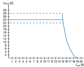
CP-C 24/10.0
