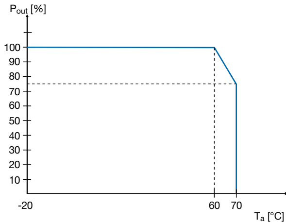
CP-E 5/3.0, CP-E 24/0.75
