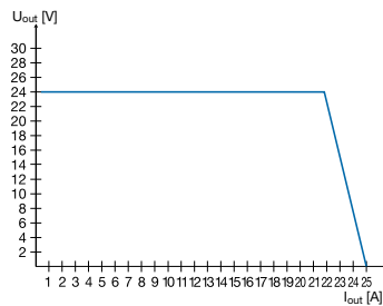
CP-S 24/20.0
