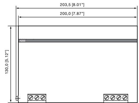
CP-S 24/20.0 CP-C 24/20.0
