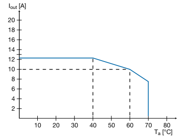
CP-S 24/10.0, CP-C 24/10.0
